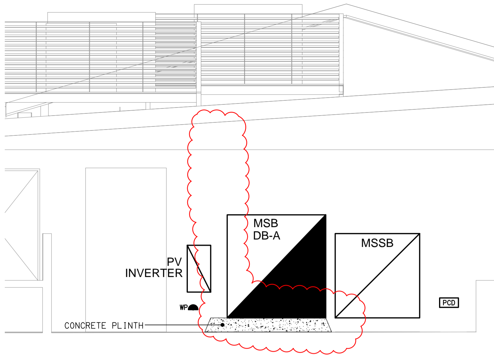
DETAIL A ELECTRICAL EQUIPMENT ELEVATION SCALE 1:50
